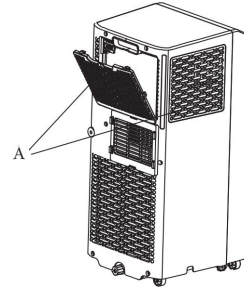
A. Evaporator air intake filter panel door
