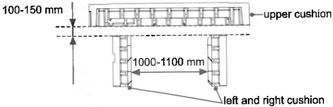
Figure 1. Top View
