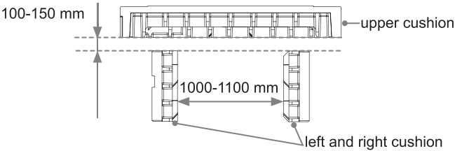
Figure 1. Top View
